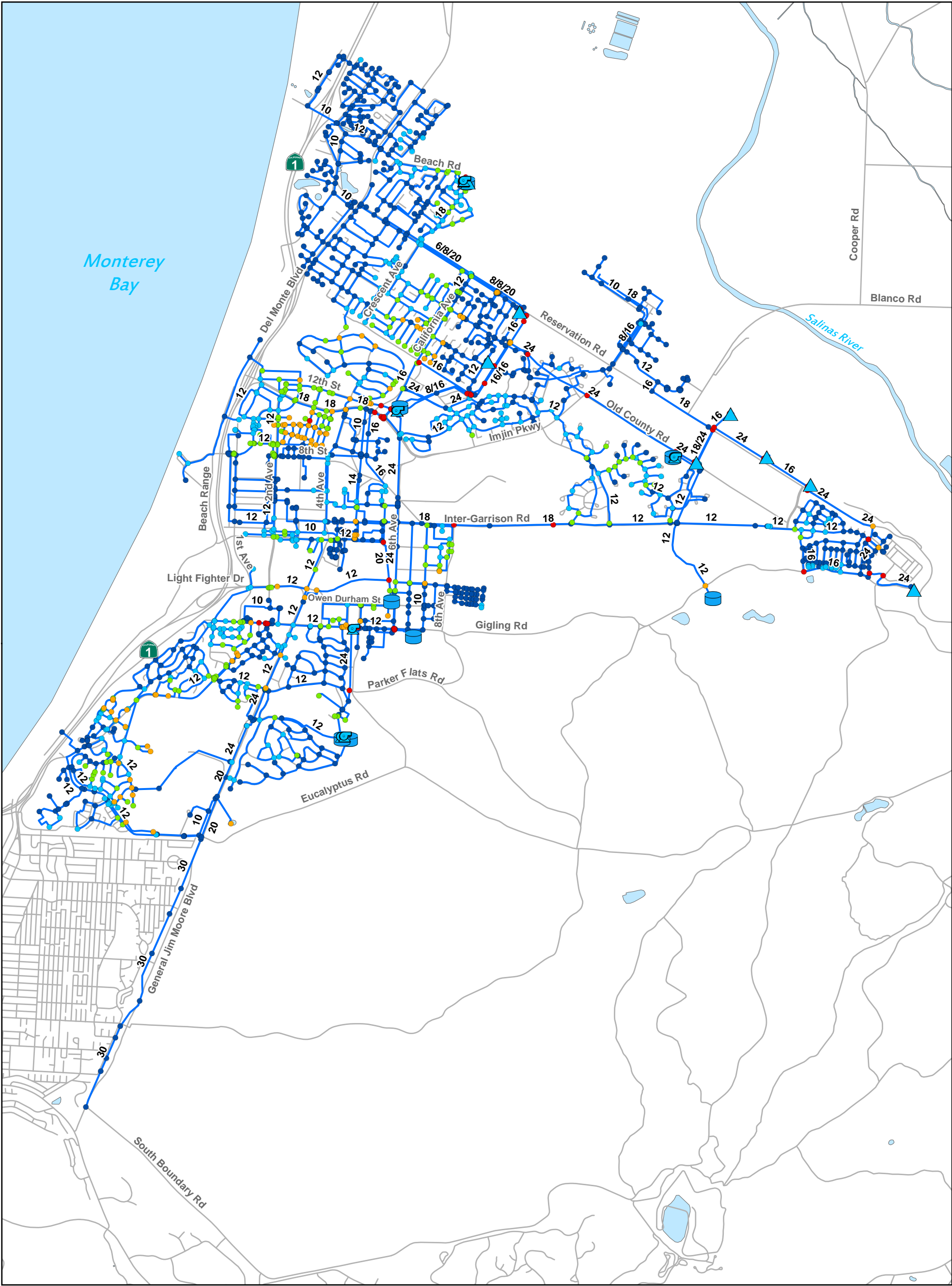
Figure 7.4 Maximum Day Pressures Water Master Plan Marina Coast Water District
