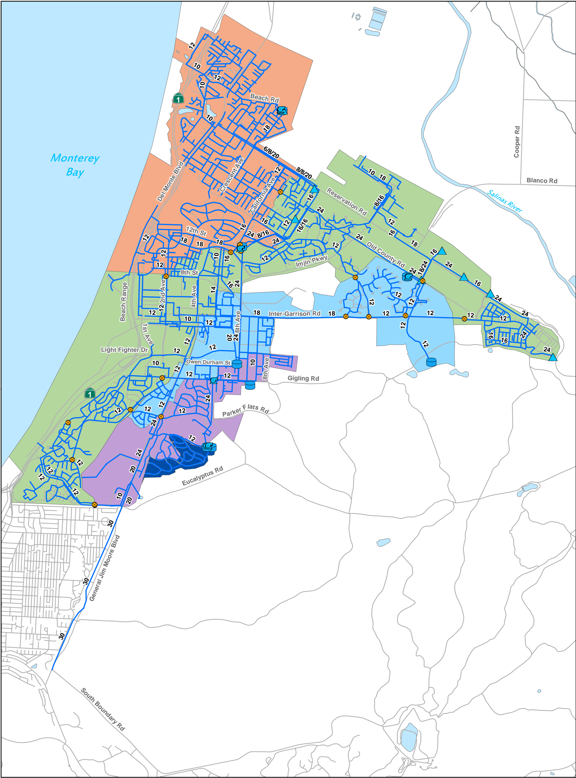
Figure 4.3 Existing Pressure Zones Water Master Plan Marina Coast Water District
