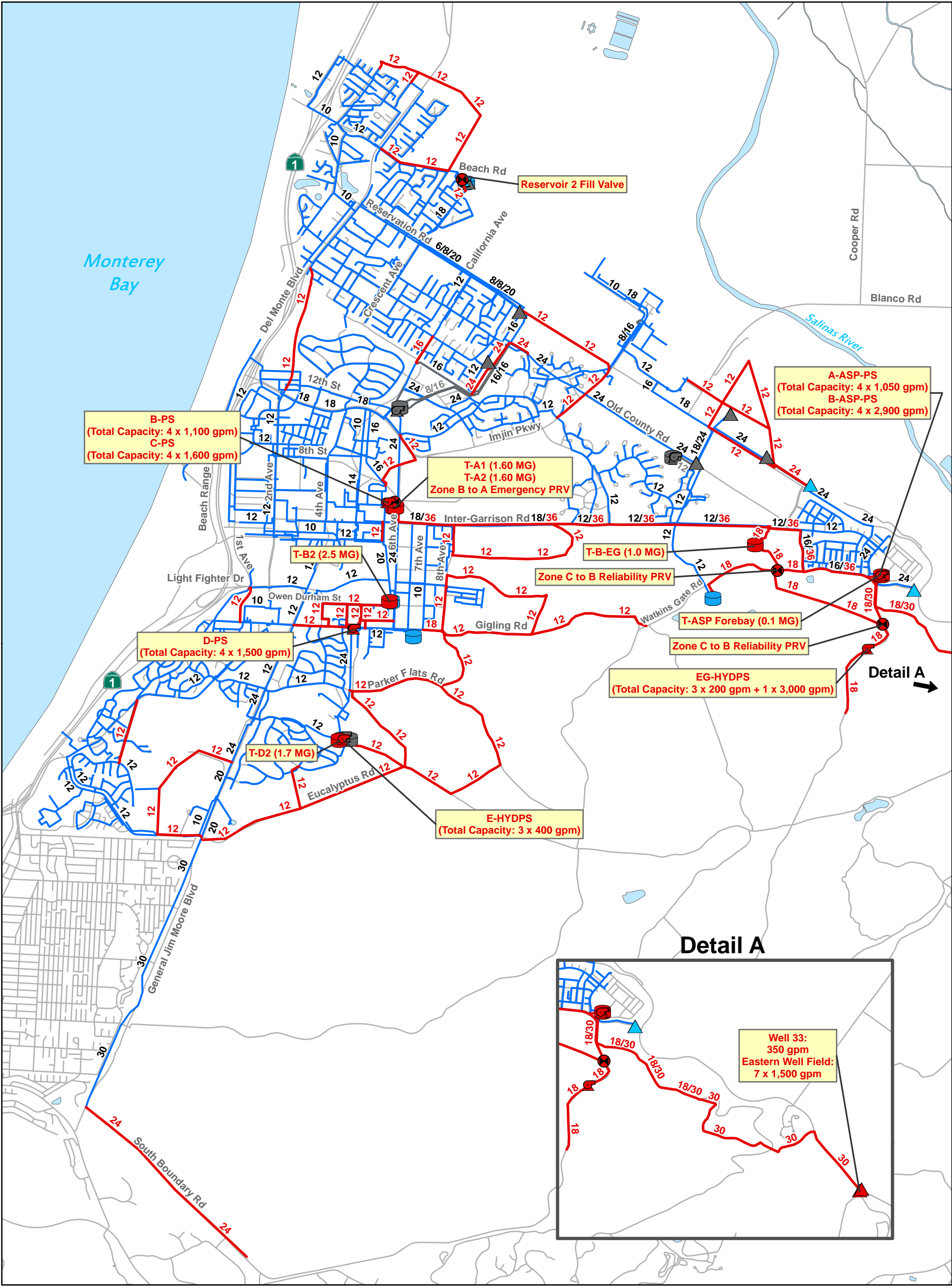
Figure 7.6 Future System Improvements Alternative 1 Water Master Plan Marina Coast Water District
