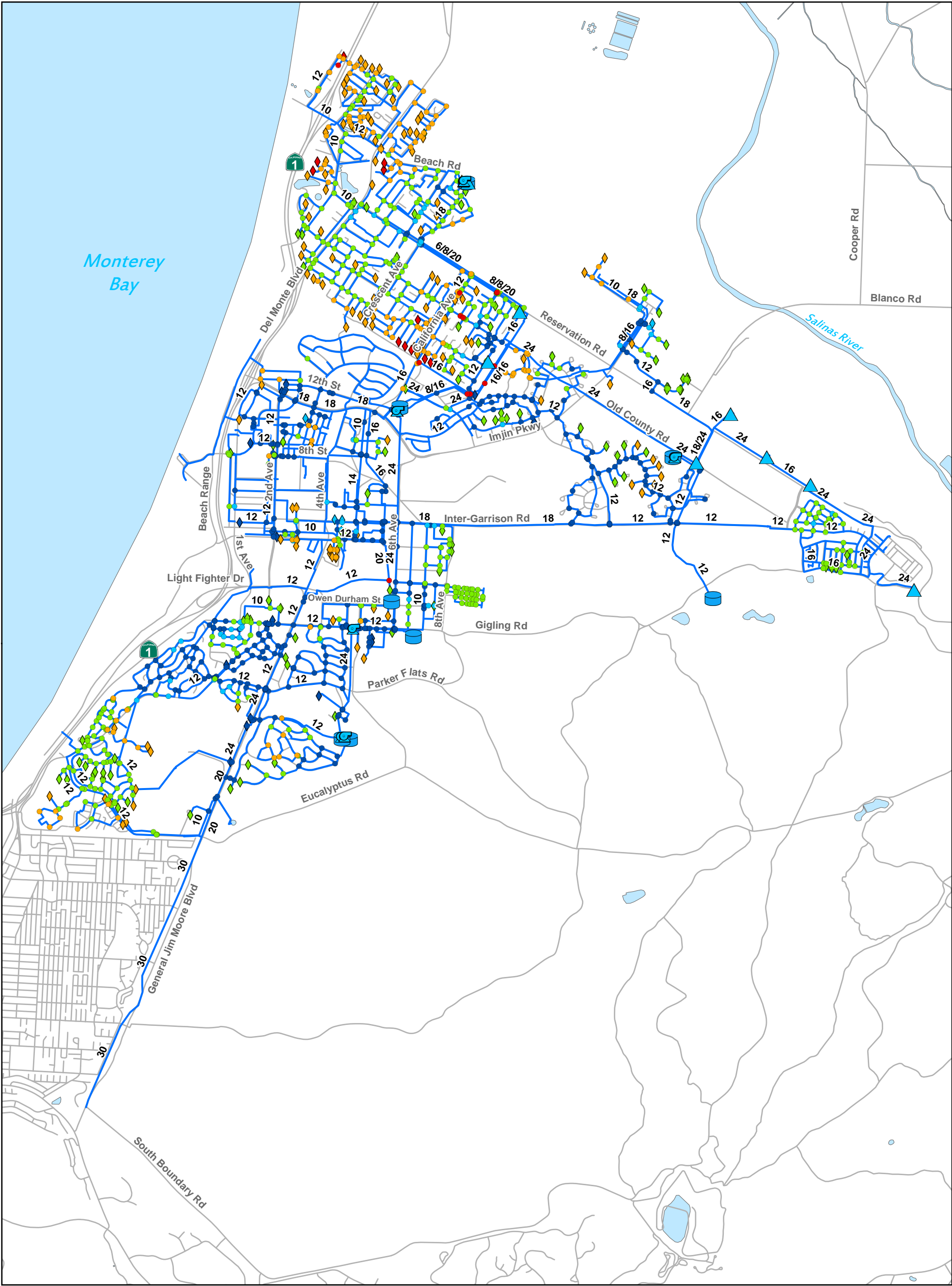
Figure 7.3 Available Fire Flow
