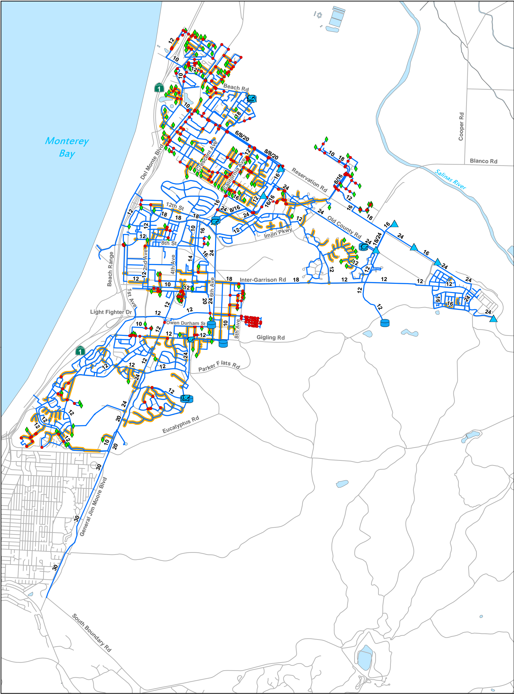
Figure 7.2 Fire Flow Analysis Water Master Plan Marina Coast Water District
