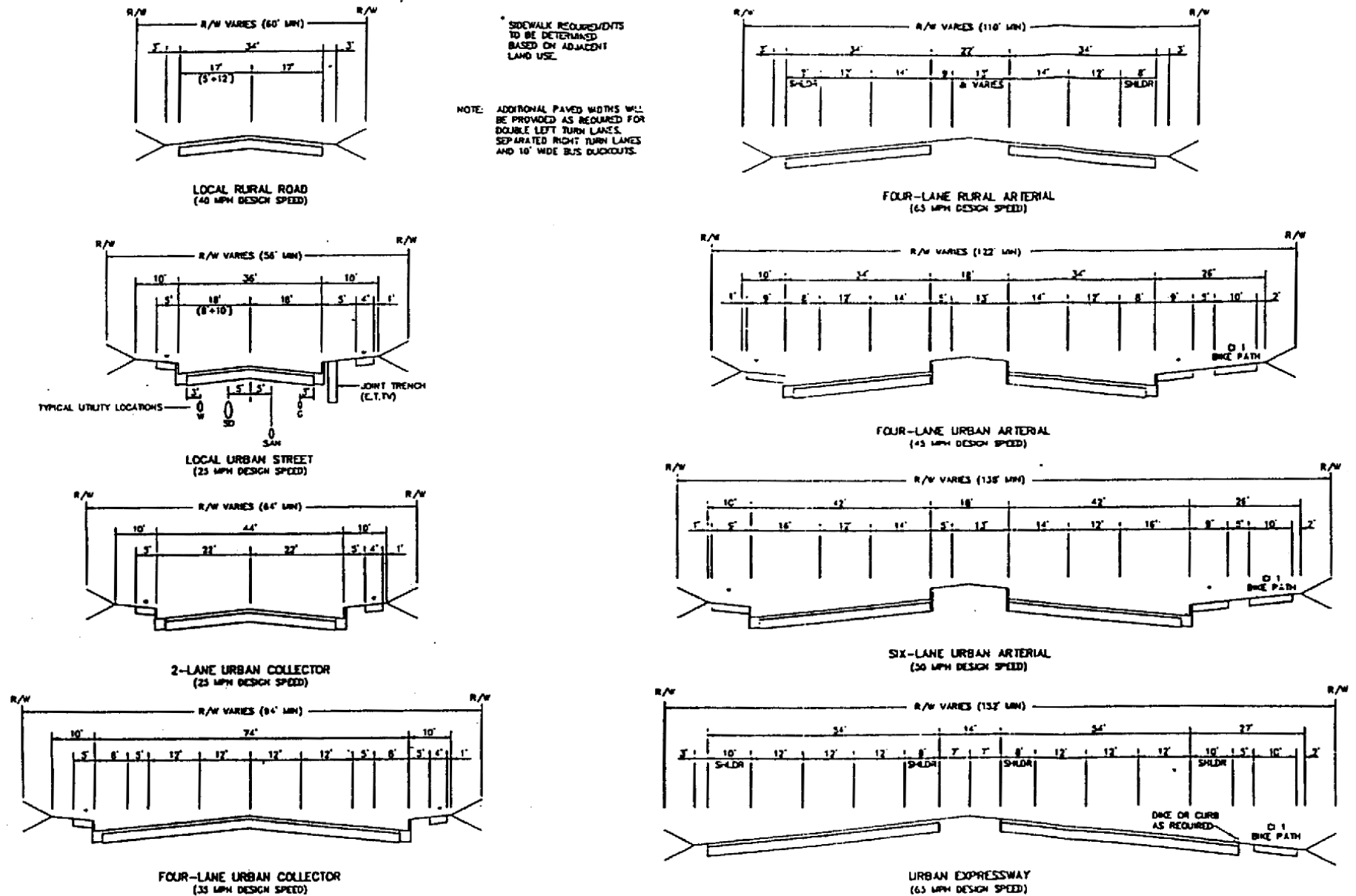
Figure 4.7-4 Roadway Design Standards
